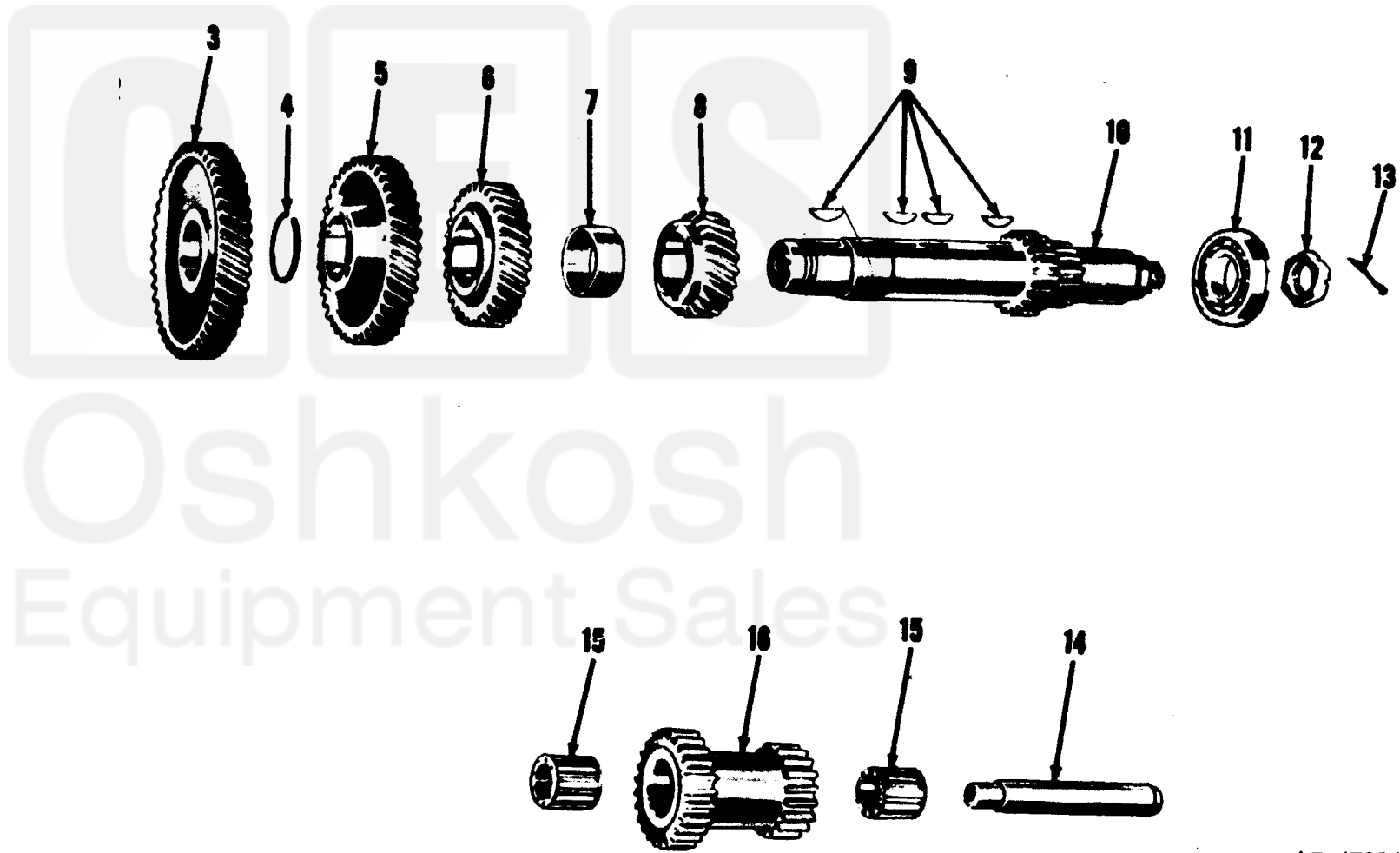
Figure 44. Transmission countershaft and idler shaft with gears—diesel.
